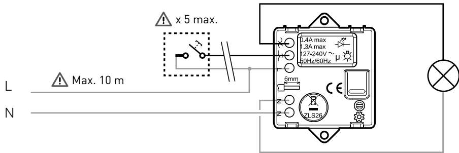
Wiring diagram
